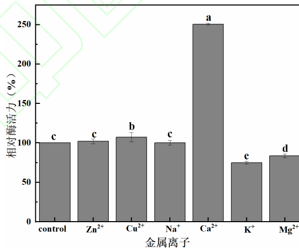
图 4 金属离子对马铃薯细胞壁果胶酶活性的影响 Fig.4 Effect of metal ions on the enzymatic activity of pectinase extracted from potato cell wall
